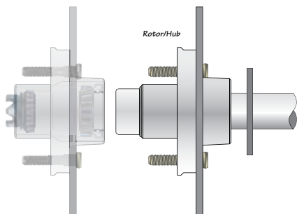
A: Install rotor/hub on spindle
