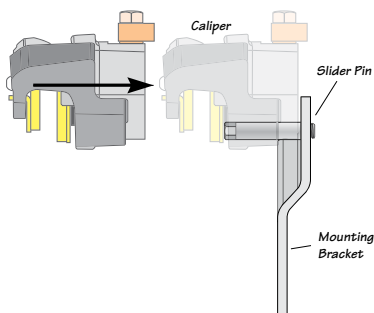
B: Install caliper on slider pins
