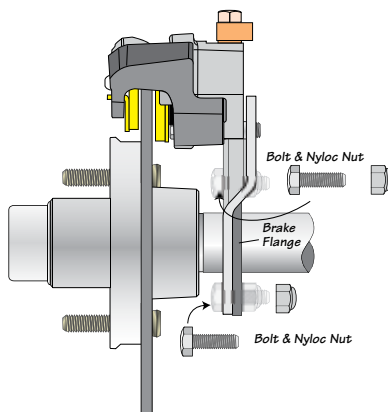
D: Bolt mounting bracket to the brake flange
