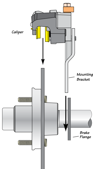
C: Slide caliper/mounting bracket over rotor
